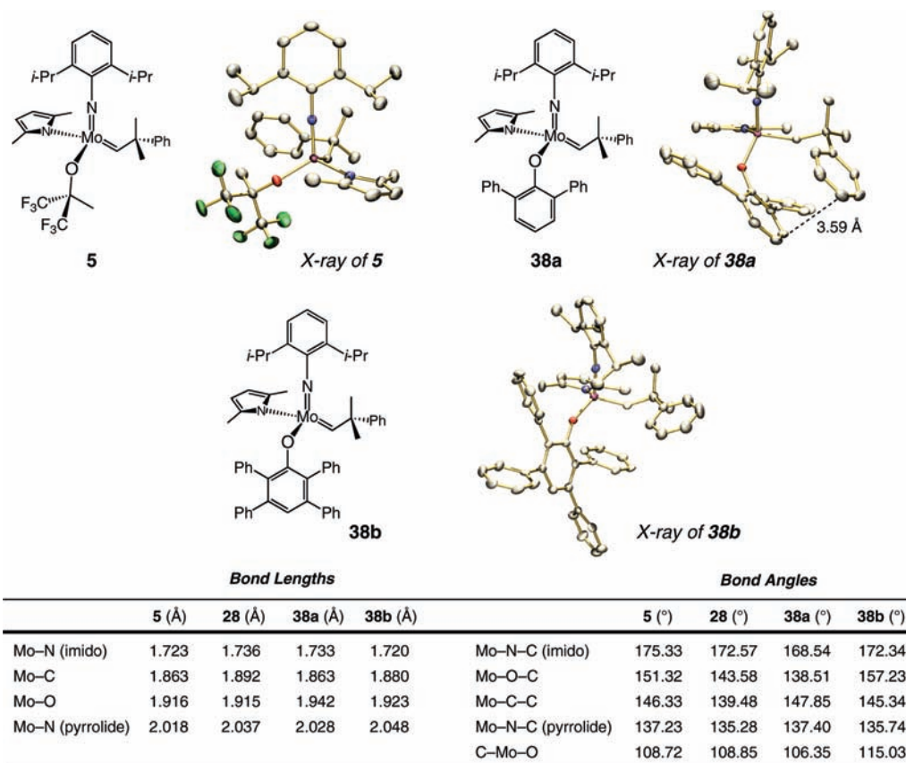
Scheme 6. X-ray Structures and Select Physical Properties of Mo-Based Monopyrrolides a
