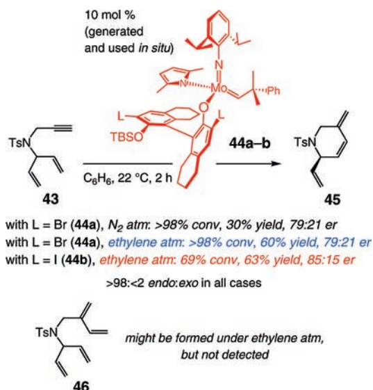
Scheme 7. Mo-Catalyzed Enantioselective RCM of a Dienyne
